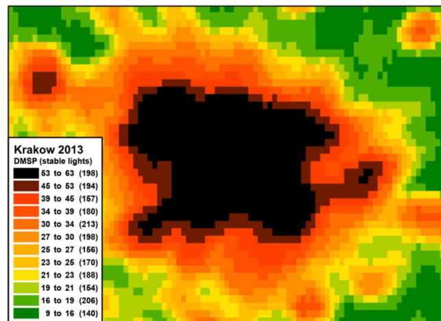
Fig. 1. DMSP annual composite. Krakow, 2013, relative units.
