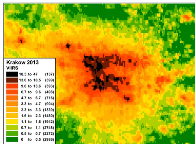
Fig. 2. VIIRS median annual composite. Krakow, 2013, nW/cm 2 /sr.
