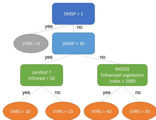
Fig. 7. Decision tree for regression
