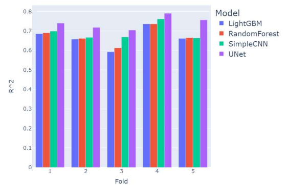
Fig. 8. R^2 (coefficient of determination) comparison between the ML models across different folds of cross-validation.
