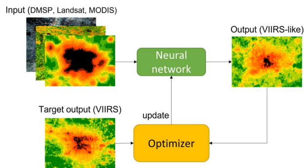
Fig. 3. Training CNN models
