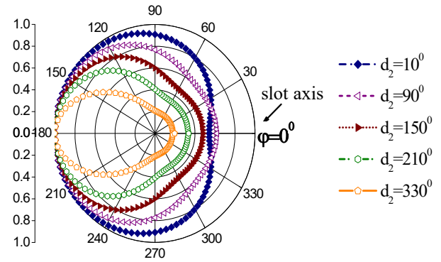
Fig. 3. Patterns of normal field distribution ( M = 1, N = 1, \gamma = 22.5^\circ, \theta = 60^\circ ).
