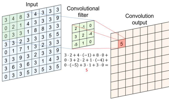
Fig. 4. Convolution operation
