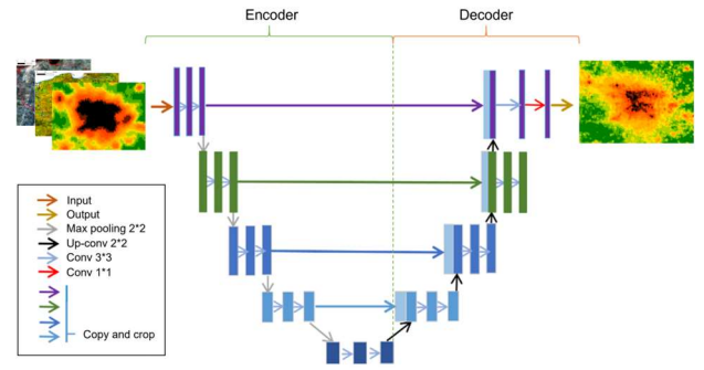
Fig. 5. UNet architecture
