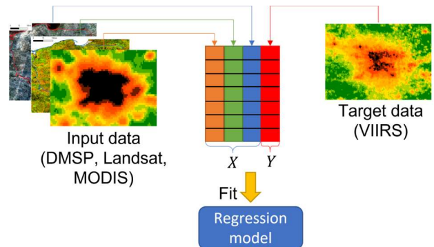
Fig. 6. Regression approach
